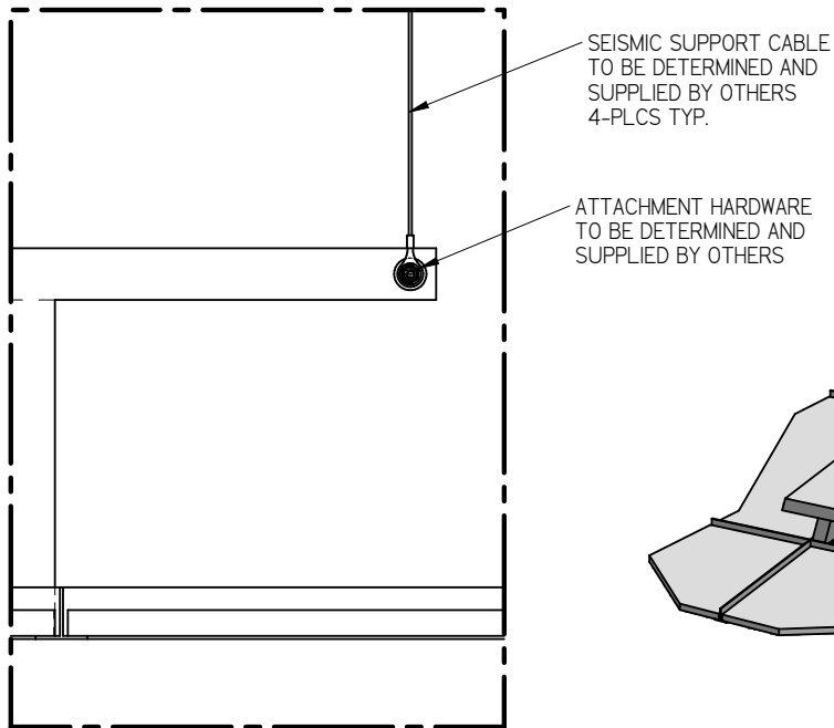
SEISMIC SUPPORT CABLE DETAIL
